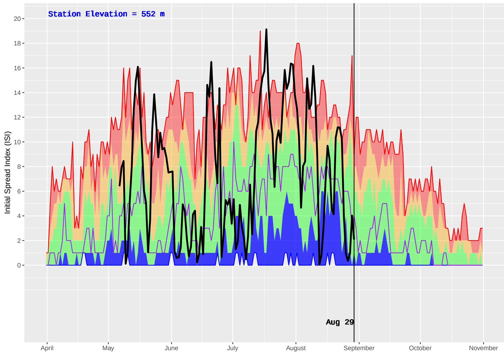
NAHATLATCH (316) : Historical (2001–2016) and Current (2018) Daily Initial Spread Index (ISI)
